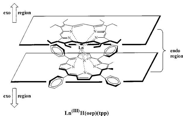
Figure 1. Schematic representation of the asymmetric \text{LnH(oep)(tpp)} complexes
