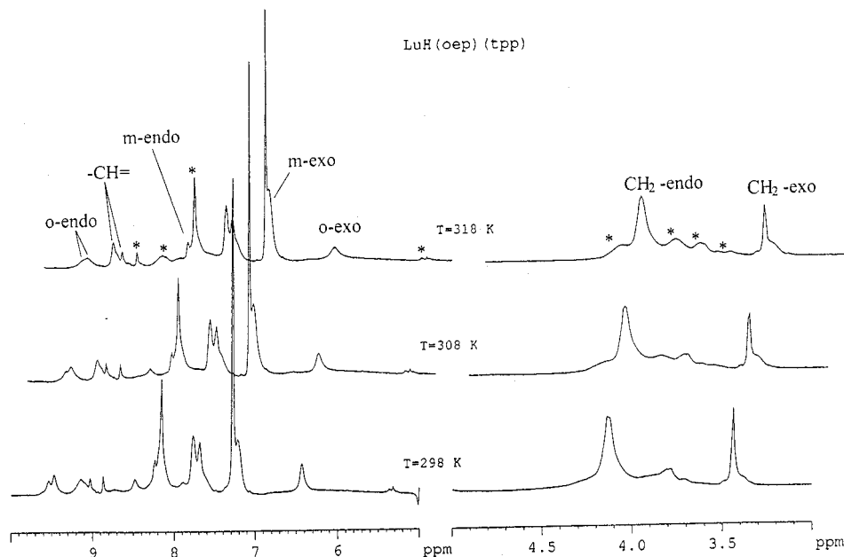
Figure 2. 500-MHz ^1\text{H} NMR spectra of \text{LuH(oep)(tpp)} (complex II ) in \text{CDCl}_3 solution at various temperatures
